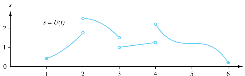
Figure 11.2: A piecewise continuous function U over the interval [1, 6]
