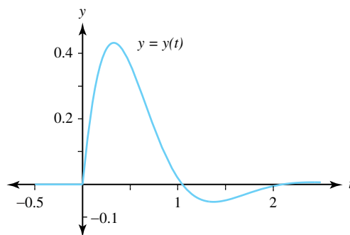
Figure 11.31: The solution y = y(t) to Example 11.32
